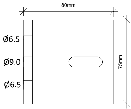
Detail 1 - GLYDE Universal Bracket - Plan
